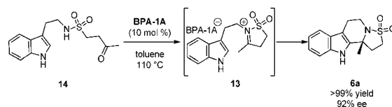
Scheme 4. Evidence for N -Sulfonyliminium Intermediate
