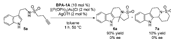
Scheme 2. Proof of Principle Study in the N -Sulfonyliminium Cyclization Cascade
